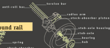
rear wheel assembly
